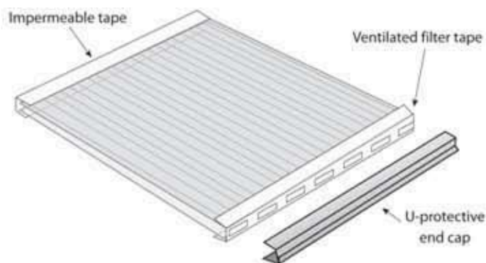
Figure 17c. Installation of Impermeable Tape at Top of the Sheet and Installation of Ventilated Tape at the Bottom of the Sheet
